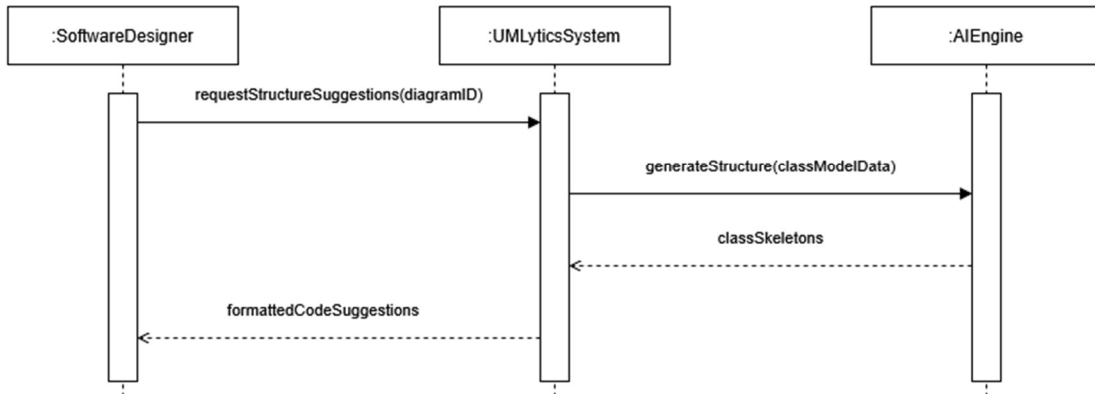
SSD: Generate Class Structure Suggestions
