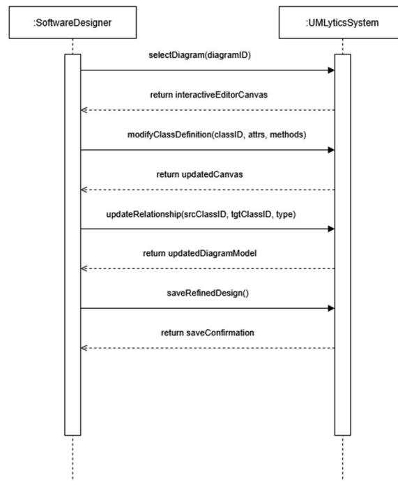
SSD: Refine UML Diagram Design
