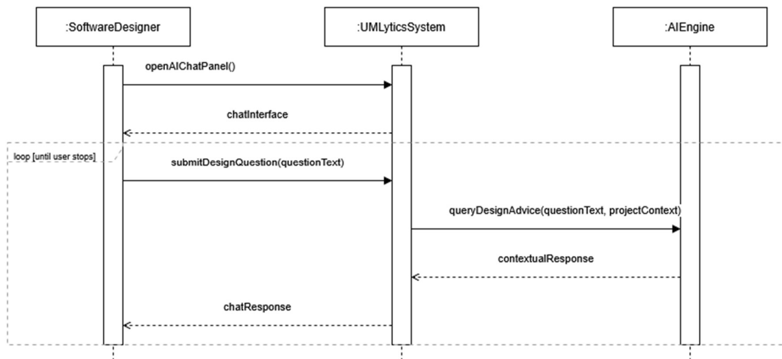
SSD: Consult AI for Design Guidance
