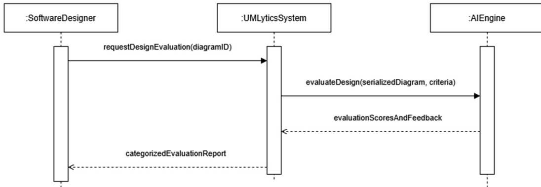
SSD: Evaluate UML Design Quality
