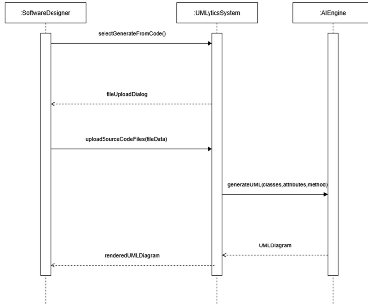
SSD: Generate UML Diagram from Source Code
