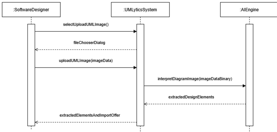
SSD: Analyze Uploaded UML Diagram
